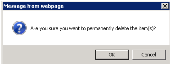
Figure 14 - Delete Confirmation
